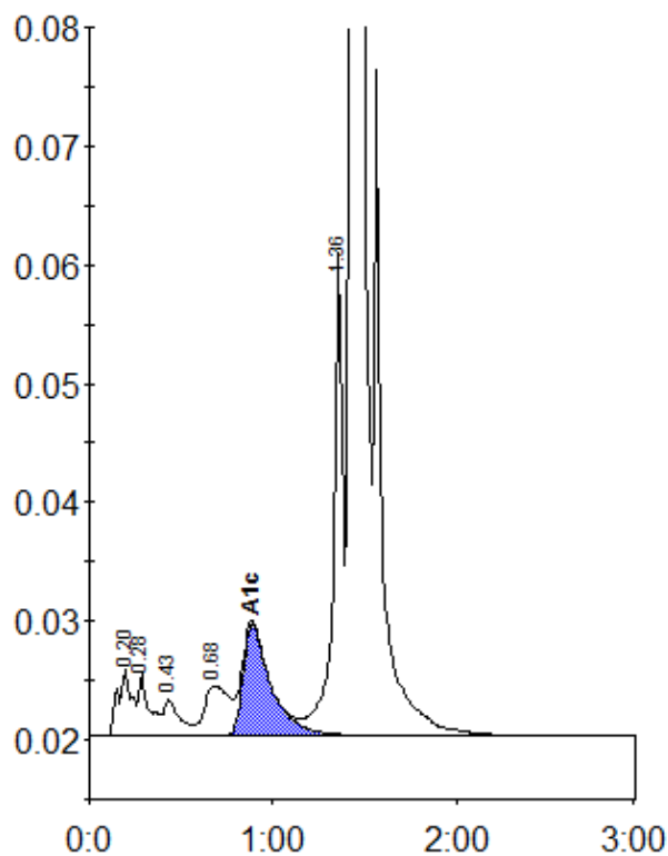
Peak table - ID: 10436937
